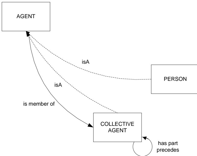
Figure 5.5 Agent Relationships
